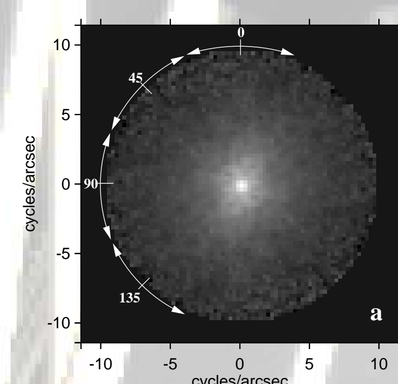
Fig. 1: Observations of OH 26.5+0.6 on October 15, 2003, with the SAO 6m telescope. a: 2-dimensional visibility function of OH 26.5+0.6 in the K band at 2.125 \mu\text{m} . North is up and east is to the left. b: Azimuthally averaged visibility of OH 26.5+0.6 in the K band obtained from the 2D visibility shown in panel a. The four curves are the visibilities azimuthally averaged between position angles -180^\circ and -135^\circ (solid line), between -135^\circ and -90^\circ (dashed), between -90^\circ and -45^\circ (dotted), and between -45^\circ and 0^\circ (dash-dotted), respectively. For clarification, only for one of the curves representative error bars are shown. The figure illustrates that there is a marginal asymmetry towards a position angle close to 0^\circ , but given the accuracy an asymmetry of the CDS of OH 26.5+0.6 can not be concluded from the measurements presented here. c: Azimuthally averaged visibility of OH 26.5+0.6 in the K band obtained from the 2D visibility shown in panel a. The visibility shown here was derived from an azimuthal average over all position angles.
