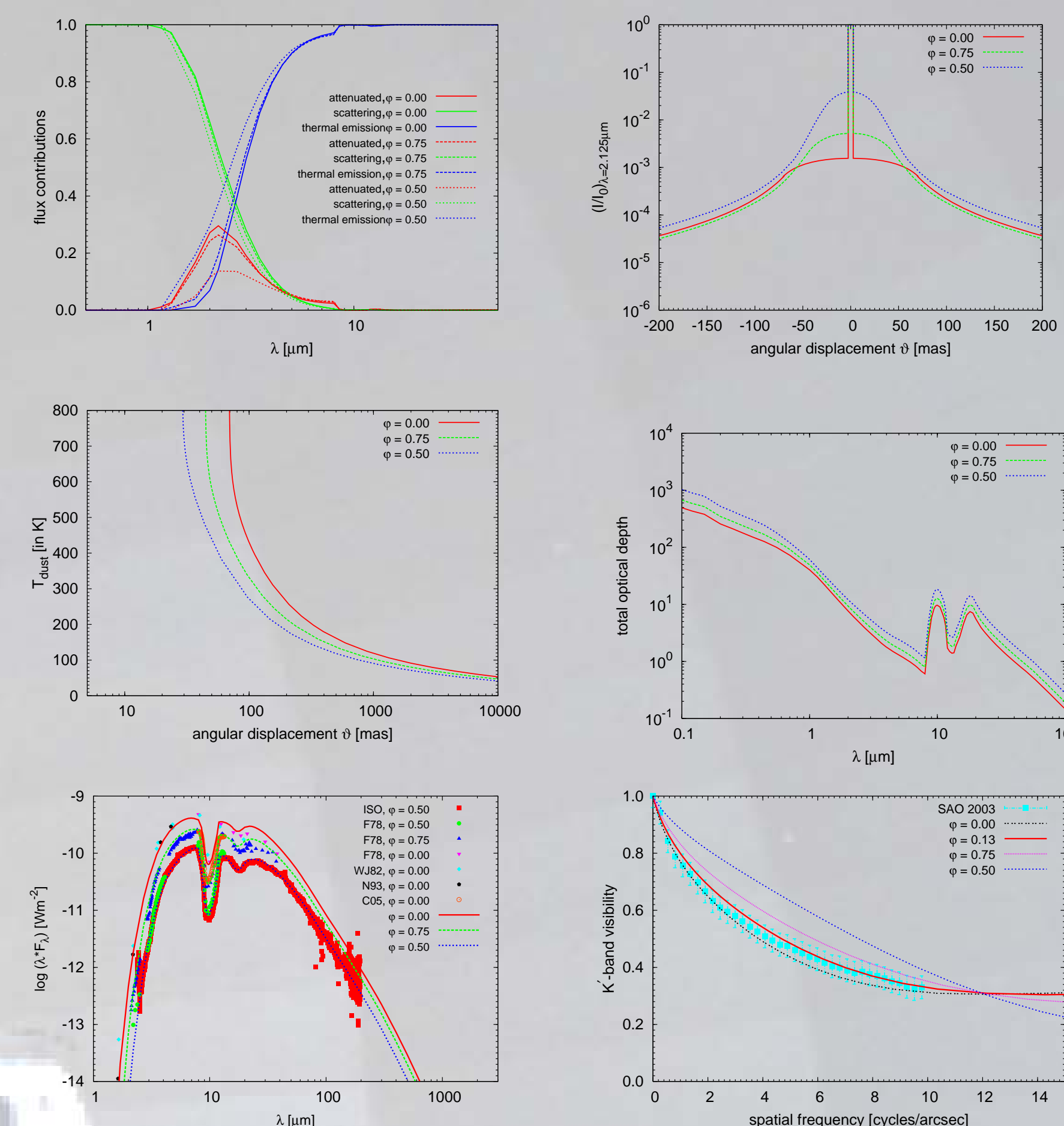
Figure 3: Variation of the dust shell properties of OH 26.5+0.6 as a function of pulsation phase (see Tab. 1). Top left: Fractional contributions to the total flux. The contribution from direct stellar light is small compared to the contribution of dust scattering and thermal emission. Top right: The normalized intensity profile at 2.125 \mu\text{m} . The sharp central peak corresponds to the central source of radiation. Middle left: Dust temperature as a function of angular distance. The point where T_{\text{dust}} = 800 \text{ K} indicates the inner radius of the dust shell. As the figure shows, due to the variability of the central source the inner dust shell boundary moves from 29.3 \text{ mas} ( = 10.1 R_{\odot} ) to 69.5 \text{ mas} ( = 27.0 R_{\odot} ) between minimum and maximum pulsation phase. Middle right: Wavelength dependence of the total optical depth. Bottom left: Spectral energy distribution. Bottom right: K -band visibility. Our 2003 measurement (filled squares) is shown for comparison with the model for phase \Phi_{\text{SAO}} = 0.13 .
